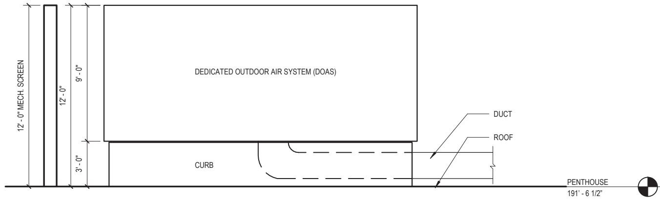
DOAS HEIGHT DIAGRAM
